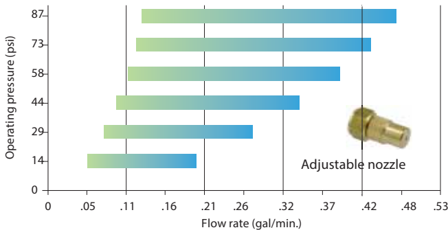
Spray performance Adjustable nozzle 1.3 mm (Flox 10 AT3, PT1 / Iris 15 AT3, PT1)
